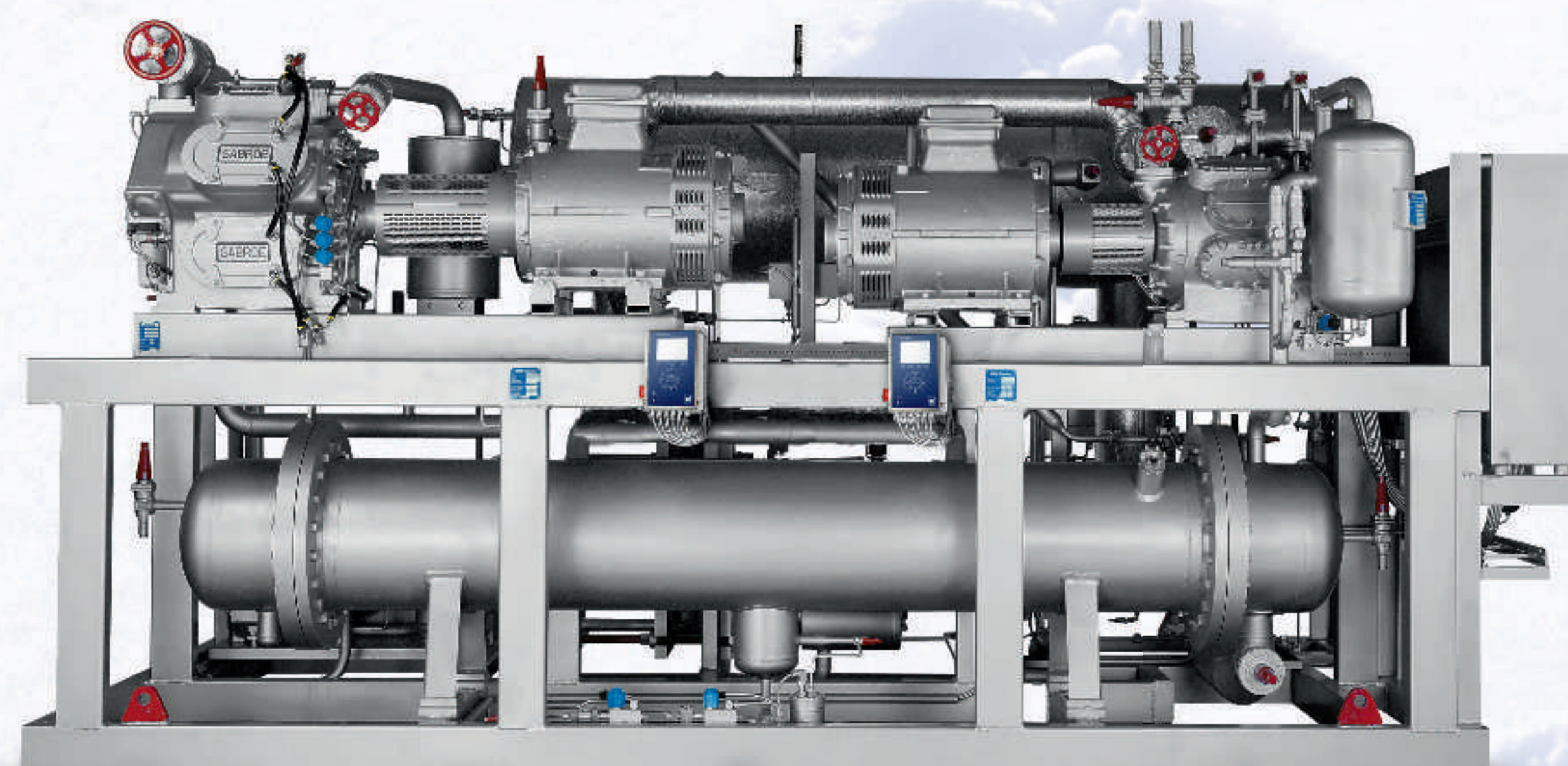
CO 2 /Ammonia Freeze Package (CAFP)
