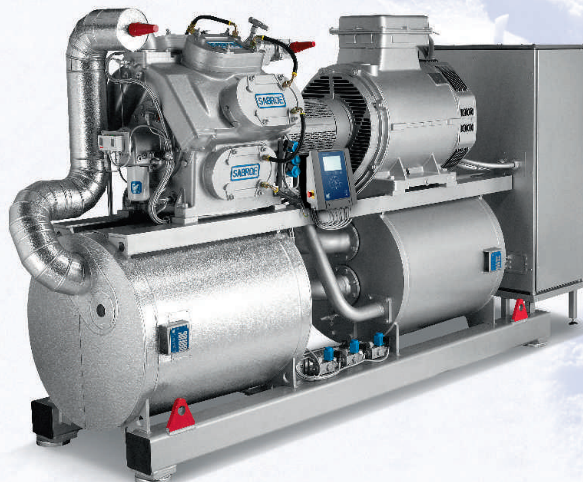
Packaged ammonia chillers (e.g. PAC, ChillPAC)
